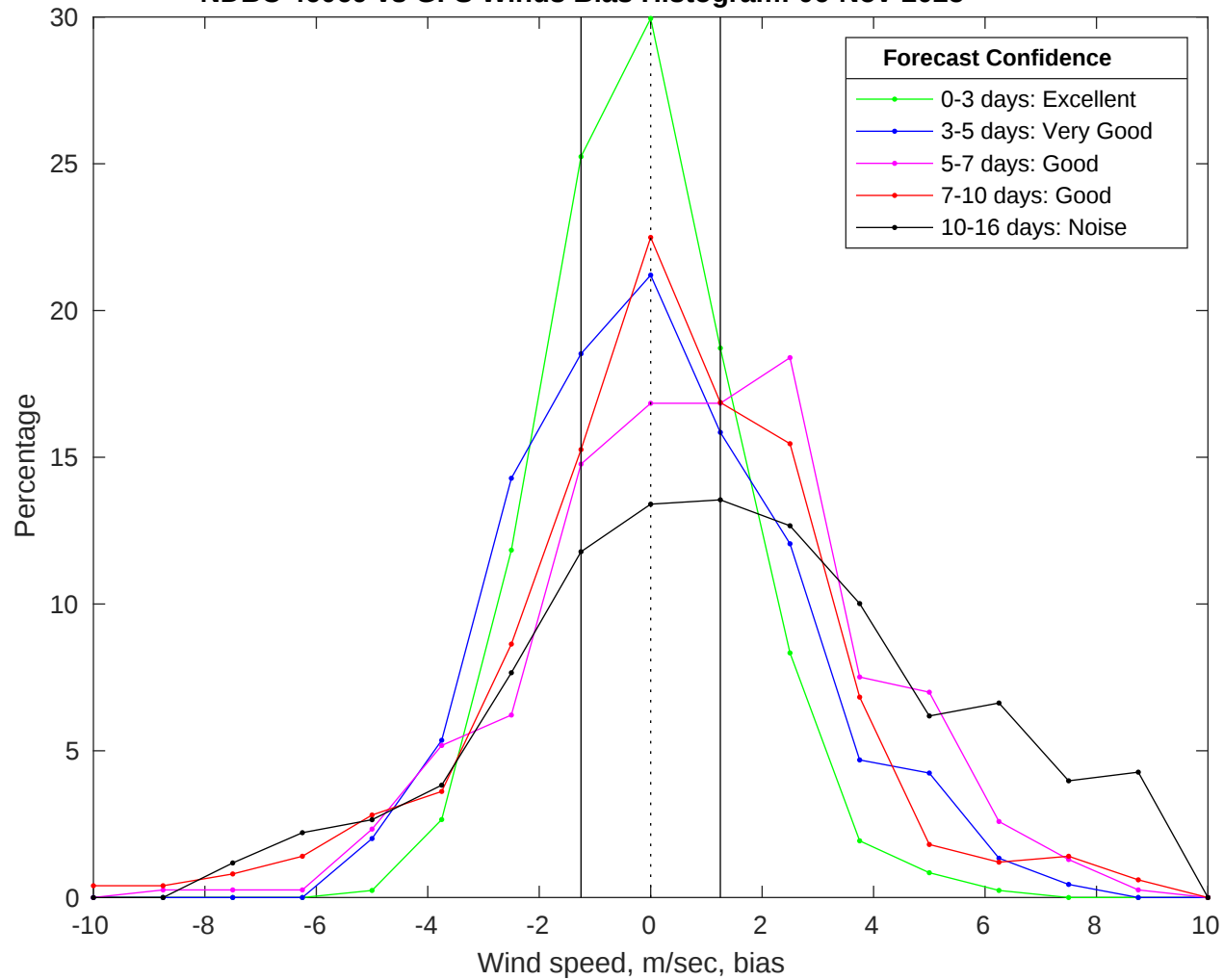
NDBC 46069 vs GFS Winds Bias Histogram: 06-Nov-2025
