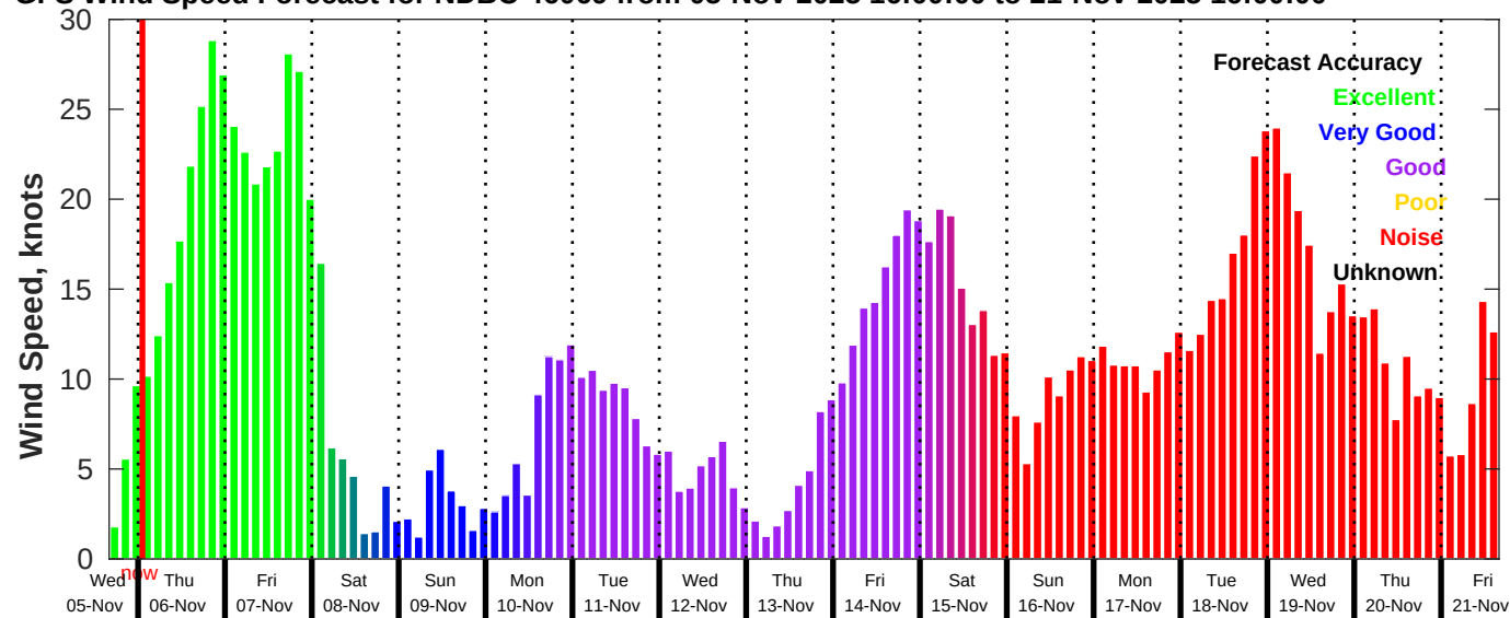
GFS Wind Speed Forecast for NDBC 46069 from 05-Nov-2025 16:00:00 to 21-Nov-2025 16:00:00
