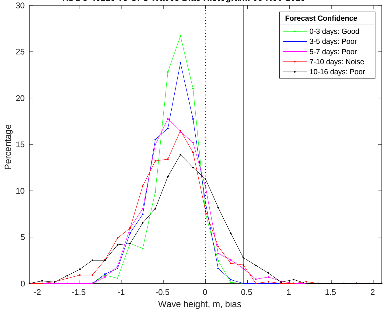
NDBC 46215 vs GFS Waves Bias Histogram: 06-Nov-2025
