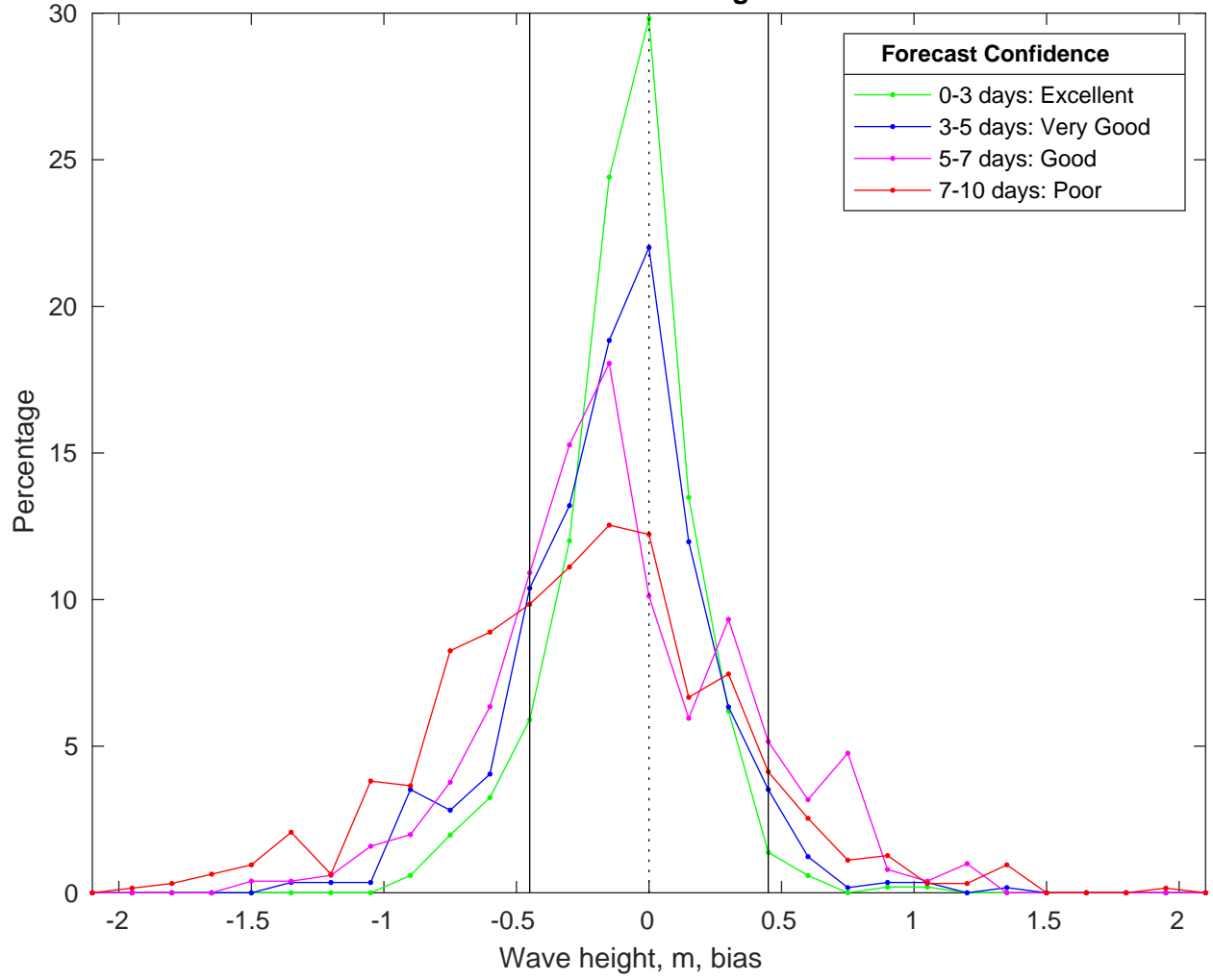
NDBC 46259 vs CMEMS Waves Bias Histogram: 06-Nov-2025
