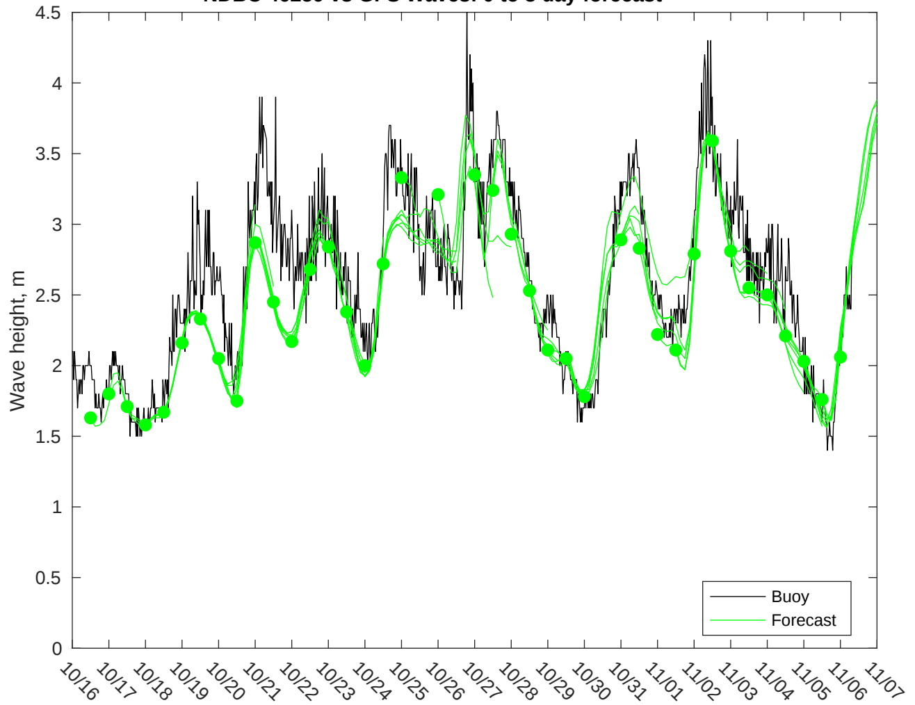
NDBC 46259 vs GFS Waves: 0 to 3 day forecast
