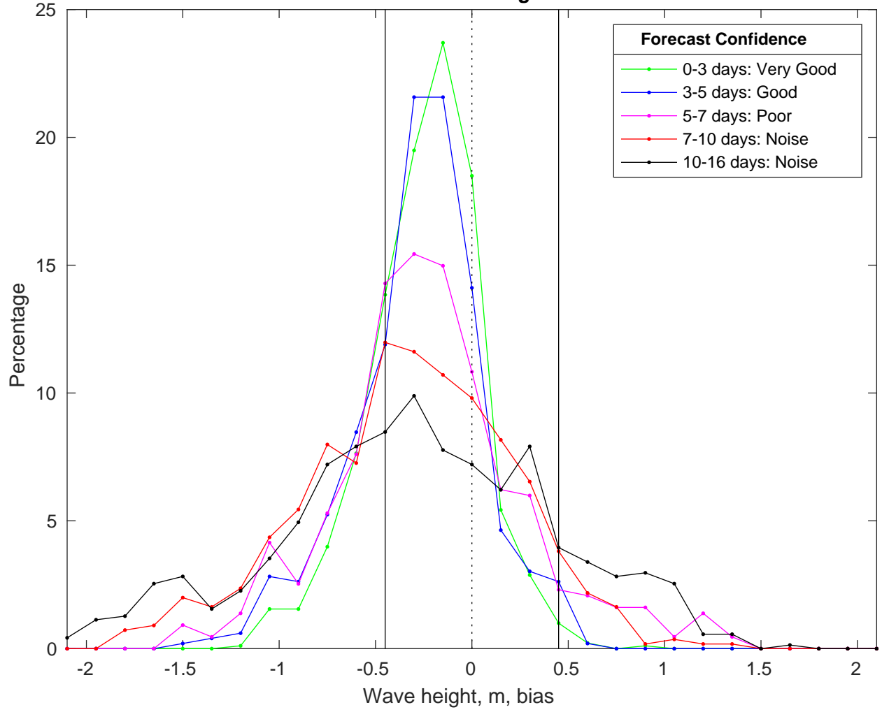
NDBC 46259 vs GFS Waves Bias Histogram: 06-Nov-2025
