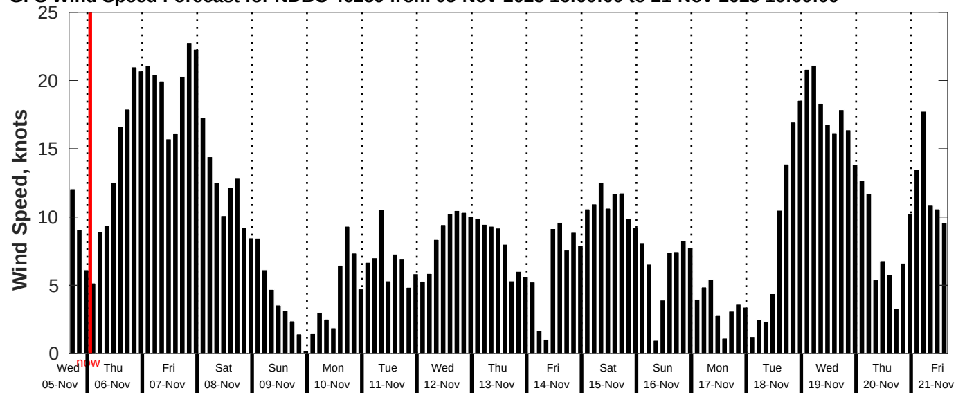
GFS Wind Speed Forecast for NDBC 46259 from 05-Nov-2025 16:00:00 to 21-Nov-2025 16:00:00
