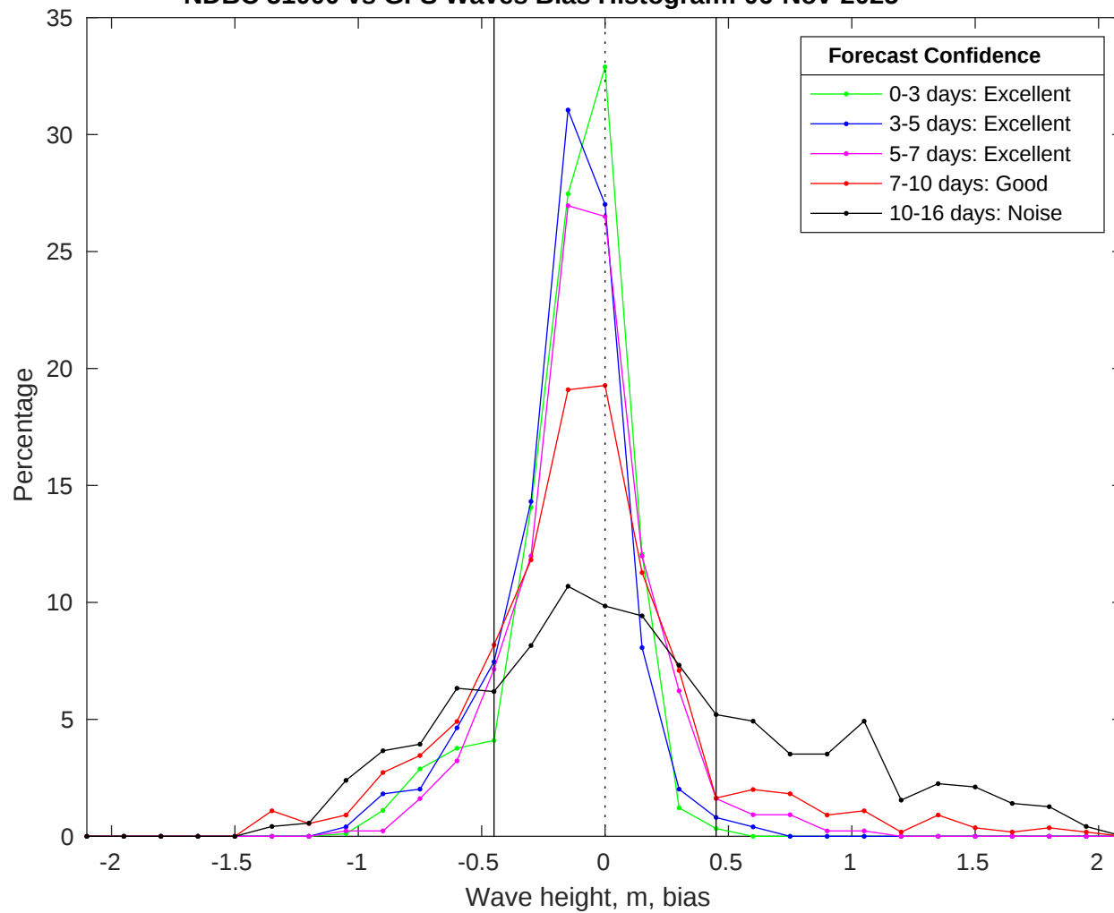
NDBC 51000 vs GFS Waves Bias Histogram: 06-Nov-2025
