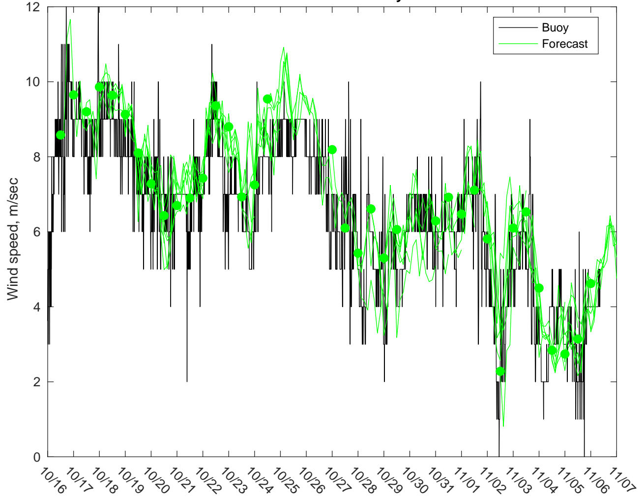
NDBC 51000 vs GFS Winds: 0 to 3 day forecast
