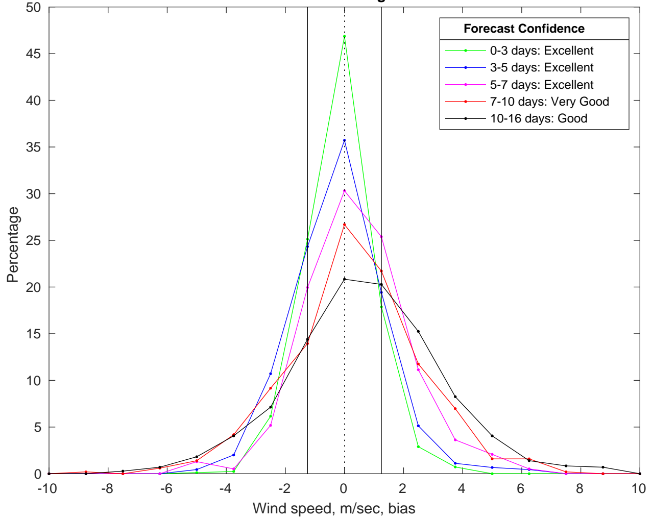
NDBC 51000 vs GFS Winds Bias Histogram: 06-Nov-2025
