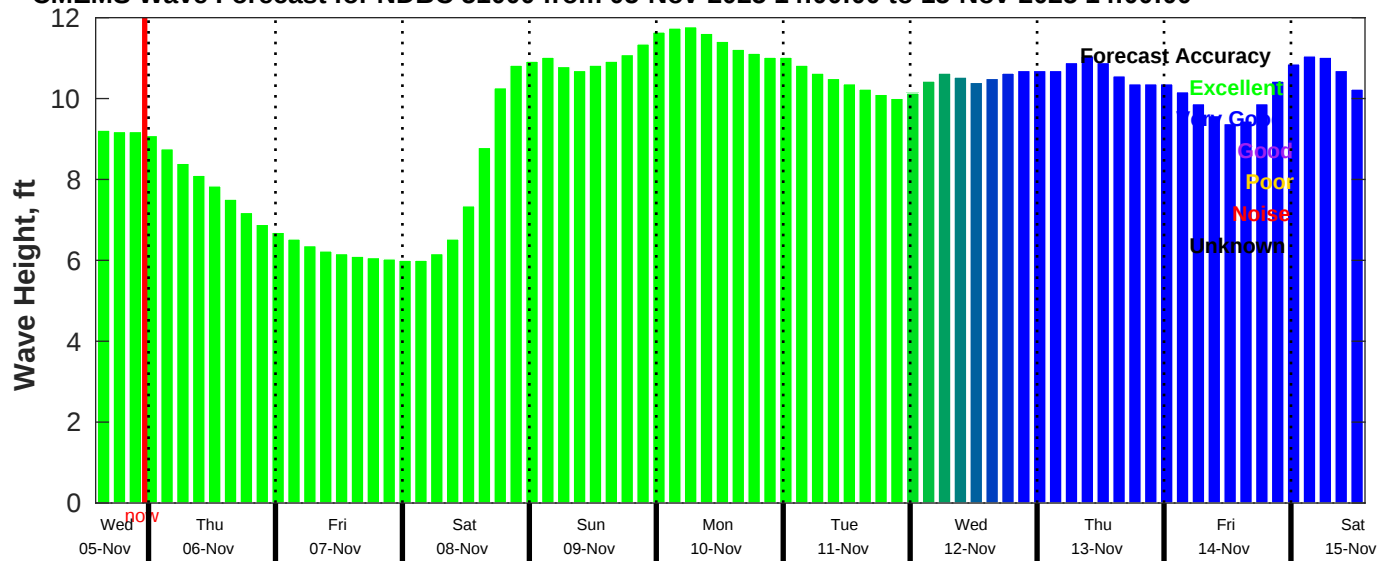
CMEMS Wave Forecast for NDBC 51000 from 05-Nov-2025 14:00:00 to 15-Nov-2025 14:00:00
