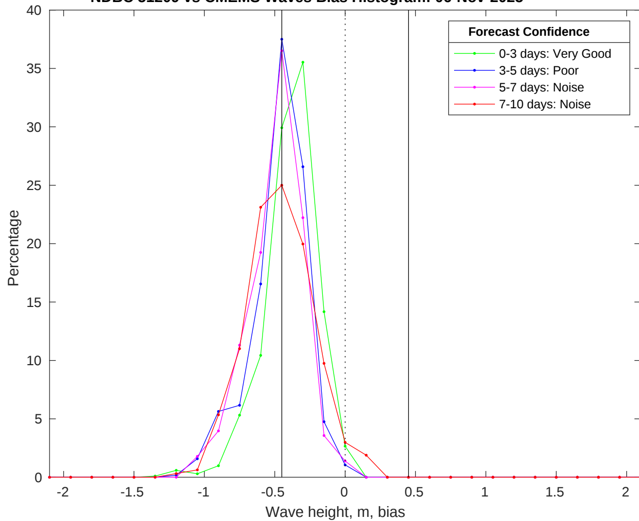
NDBC 51209 vs CMEMS Waves Bias Histogram: 06-Nov-2025
