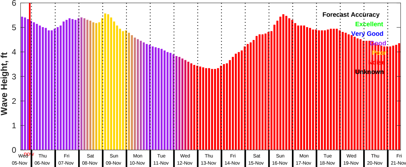
GFS Wave Forecast for NDBC 51209 from 05-Nov-2025 13:00:00 to 21-Nov-2025 13:00:00
