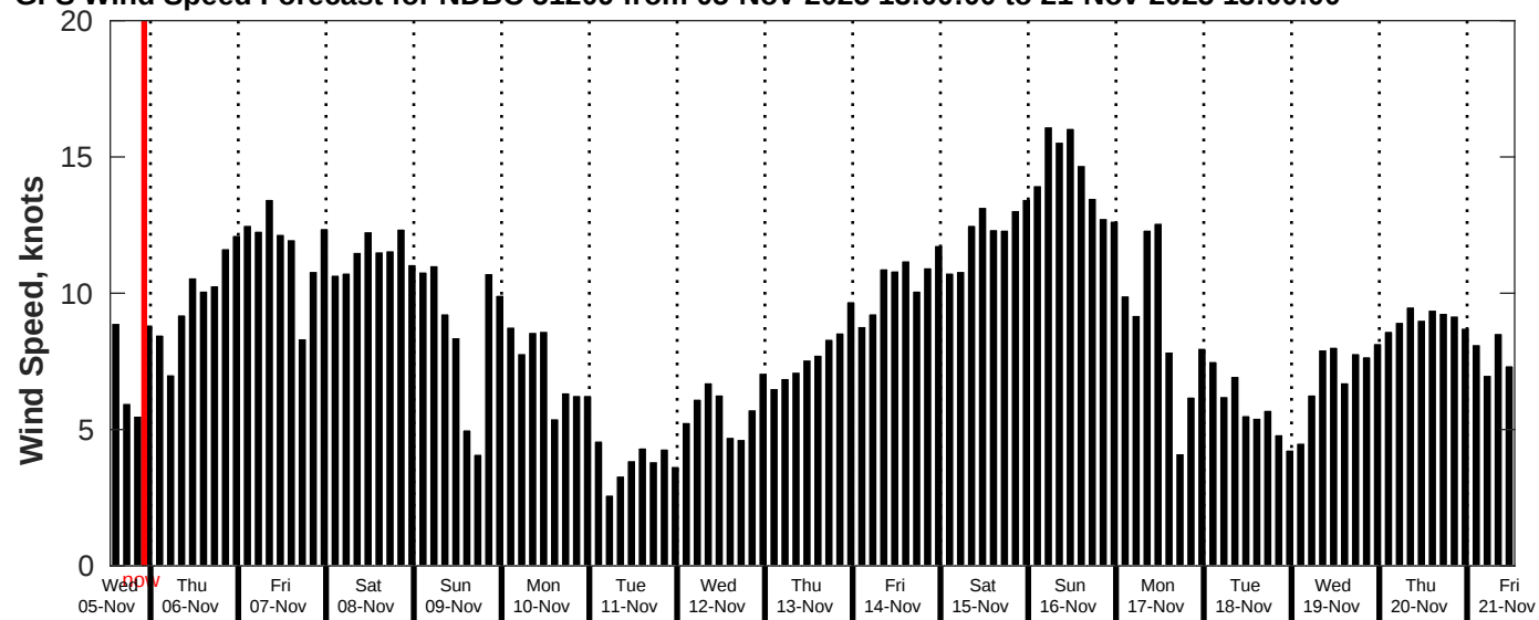
GFS Wind Speed Forecast for NDBC 51209 from 05-Nov-2025 13:00:00 to 21-Nov-2025 13:00:00
