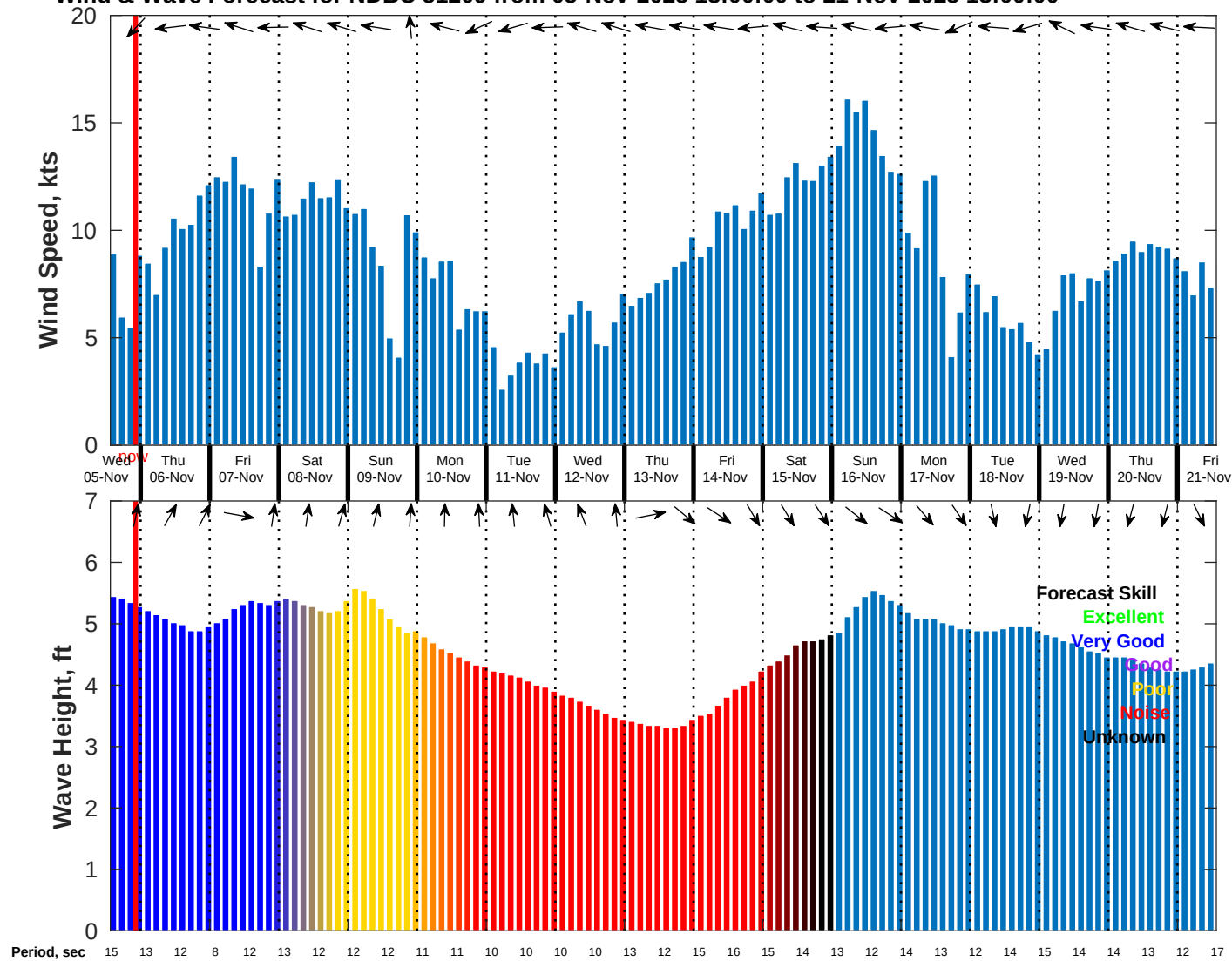
Wind & Wave Forecast for NDBC 51209 from 05-Nov-2025 13:00:00 to 21-Nov-2025 13:00:00
