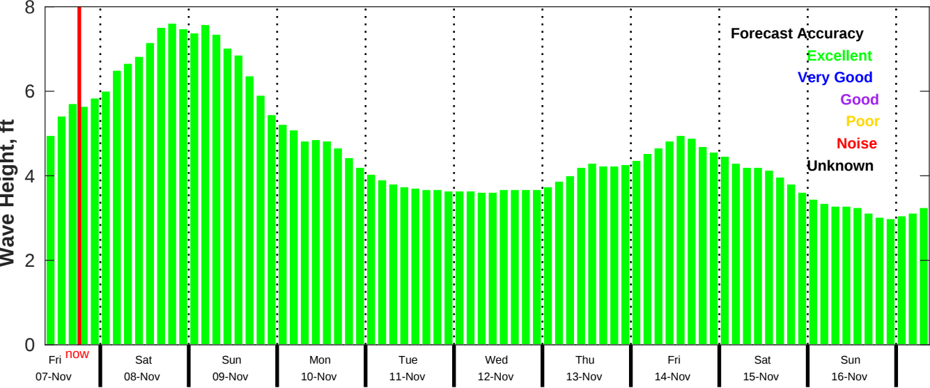
CMEMS Wave Forecast for NDBC 52212 from 06-Nov-2025 09:00:00 to 16-Nov-2025 09:00:00
