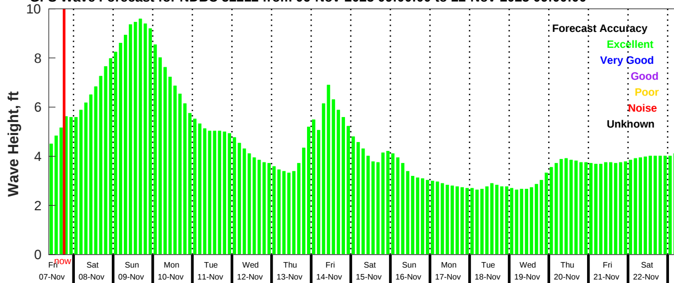
GFS Wave Forecast for NDBC 52212 from 06-Nov-2025 09:00:00 to 22-Nov-2025 09:00:00
