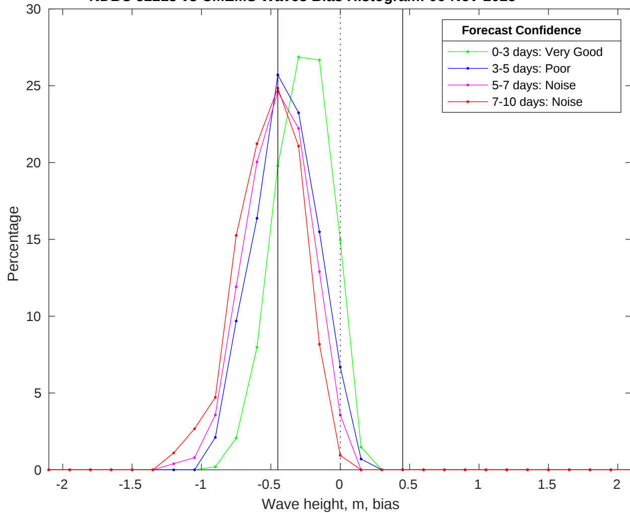
NDBC 52213 vs CMEMS Waves Bias Histogram: 06-Nov-2025
