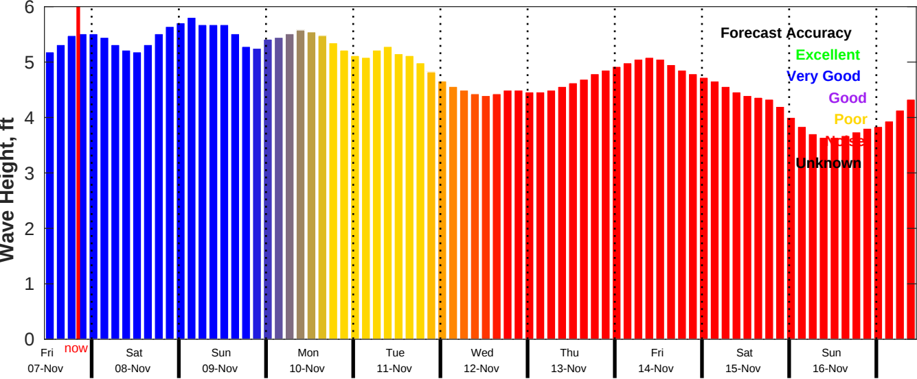
CMEMS Wave Forecast for NDBC 52213 from 06-Nov-2025 11:00:00 to 16-Nov-2025 11:00:00
