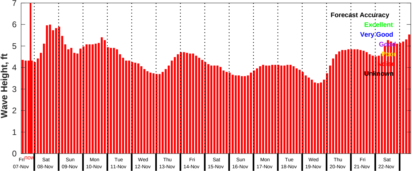
GFS Wave Forecast for NDBC 52213 from 06-Nov-2025 11:00:00 to 22-Nov-2025 11:00:00
