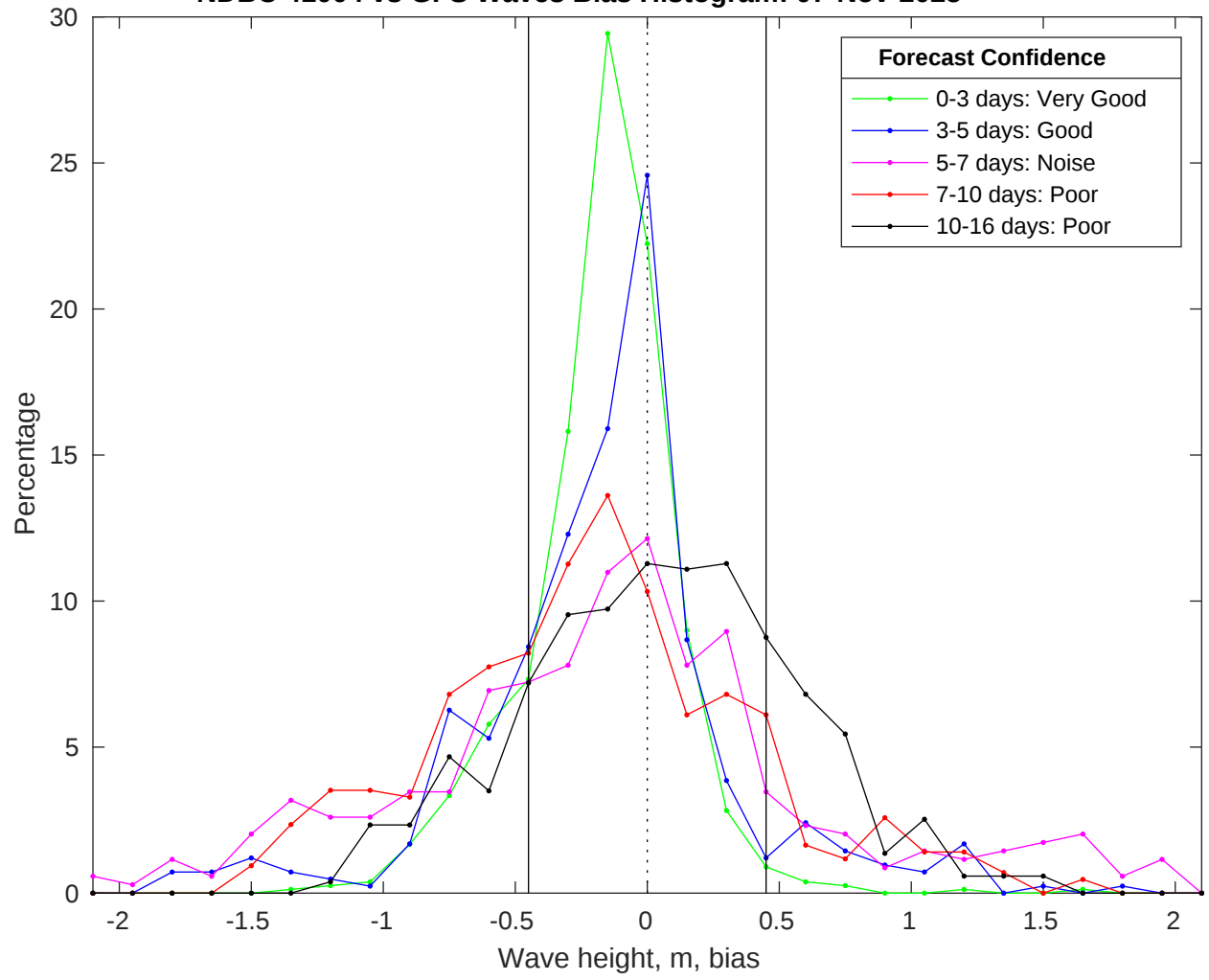
NDBC 41004 vs GFS Waves Bias Histogram: 07-Nov-2025
