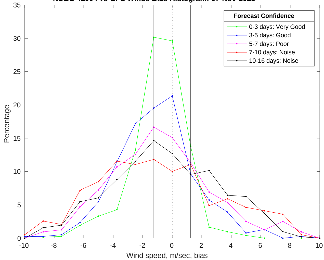
NDBC 41004 vs GFS Winds Bias Histogram: 07-Nov-2025
