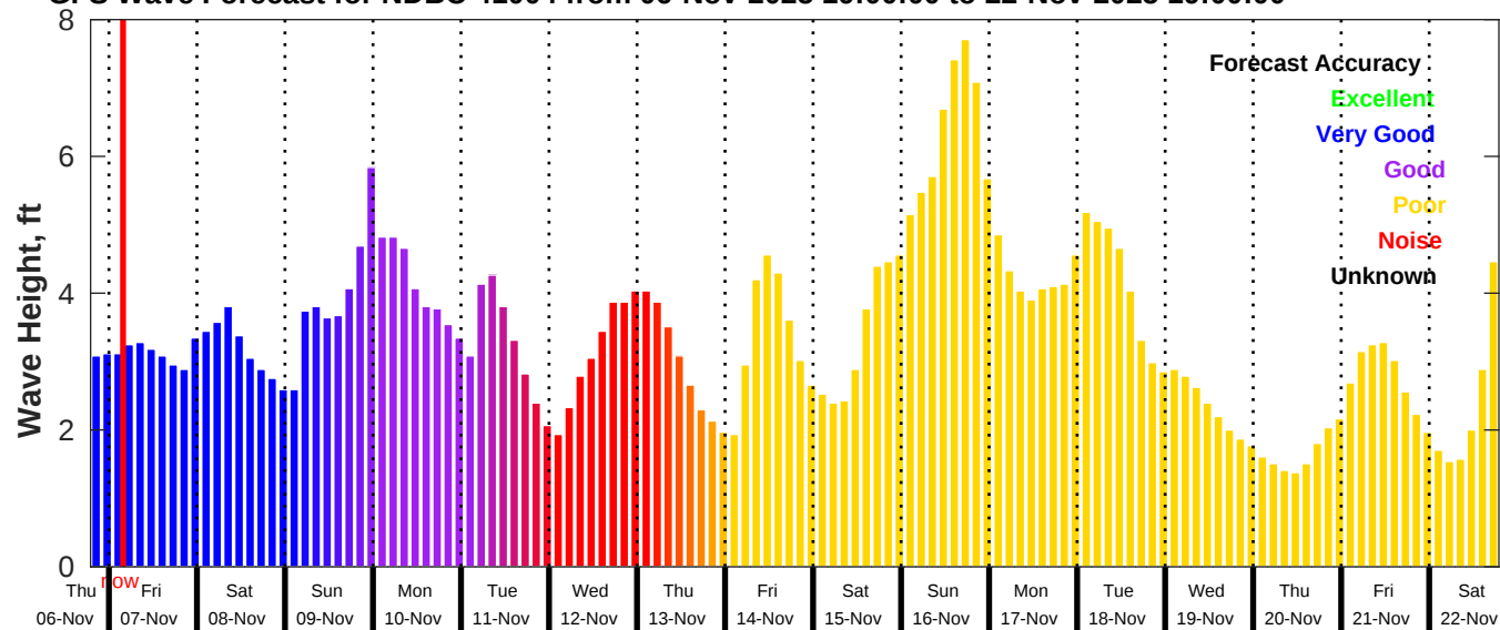
GFS Wave Forecast for NDBC 41004 from 06-Nov-2025 19:00:00 to 22-Nov-2025 19:00:00
