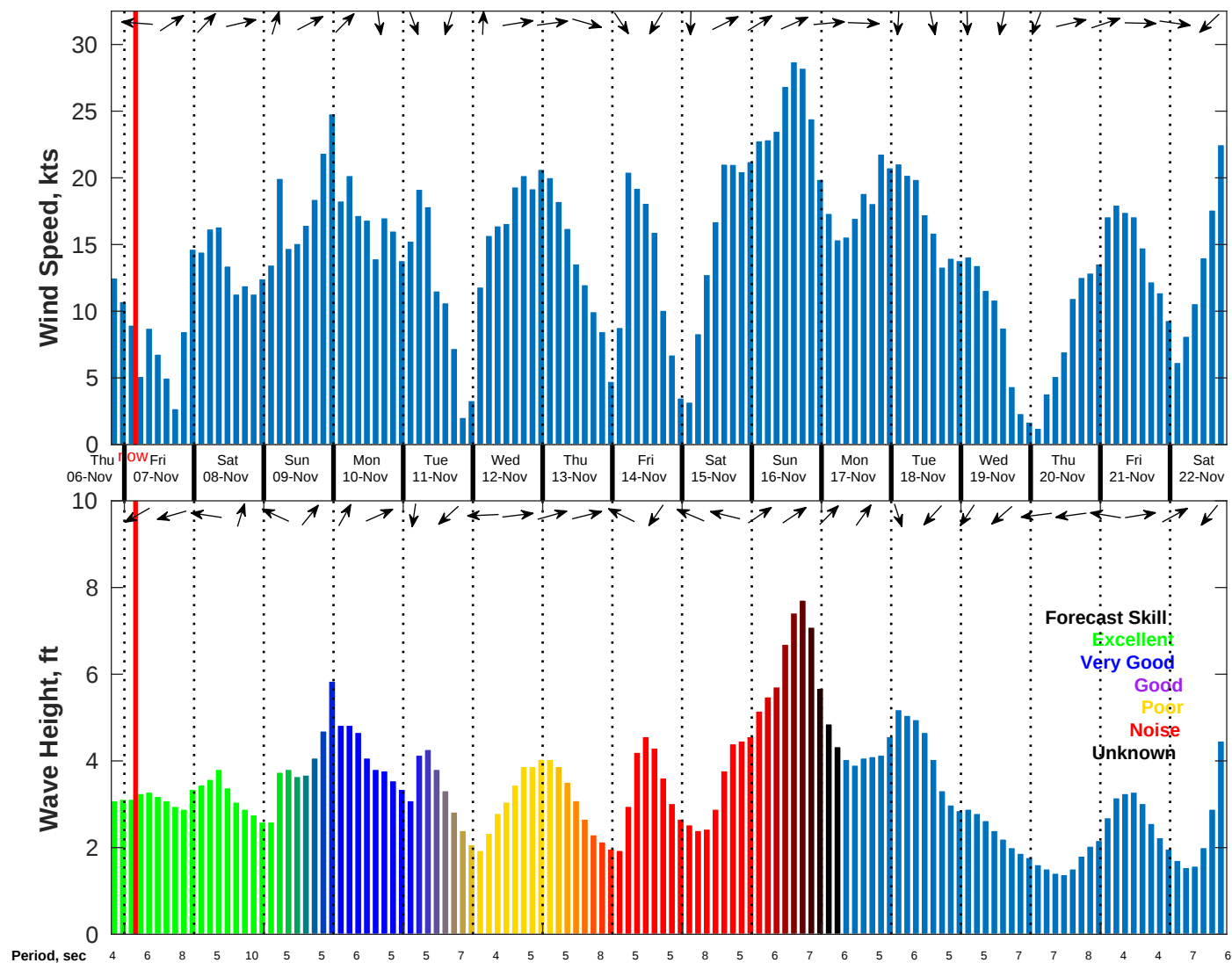
Wind & Wave Forecast for NDBC 41004 from 06-Nov-2025 19:00:00 to 22-Nov-2025 19:00:00
