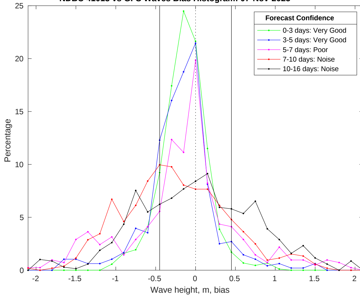
NDBC 41013 vs GFS Waves Bias Histogram: 07-Nov-2025
