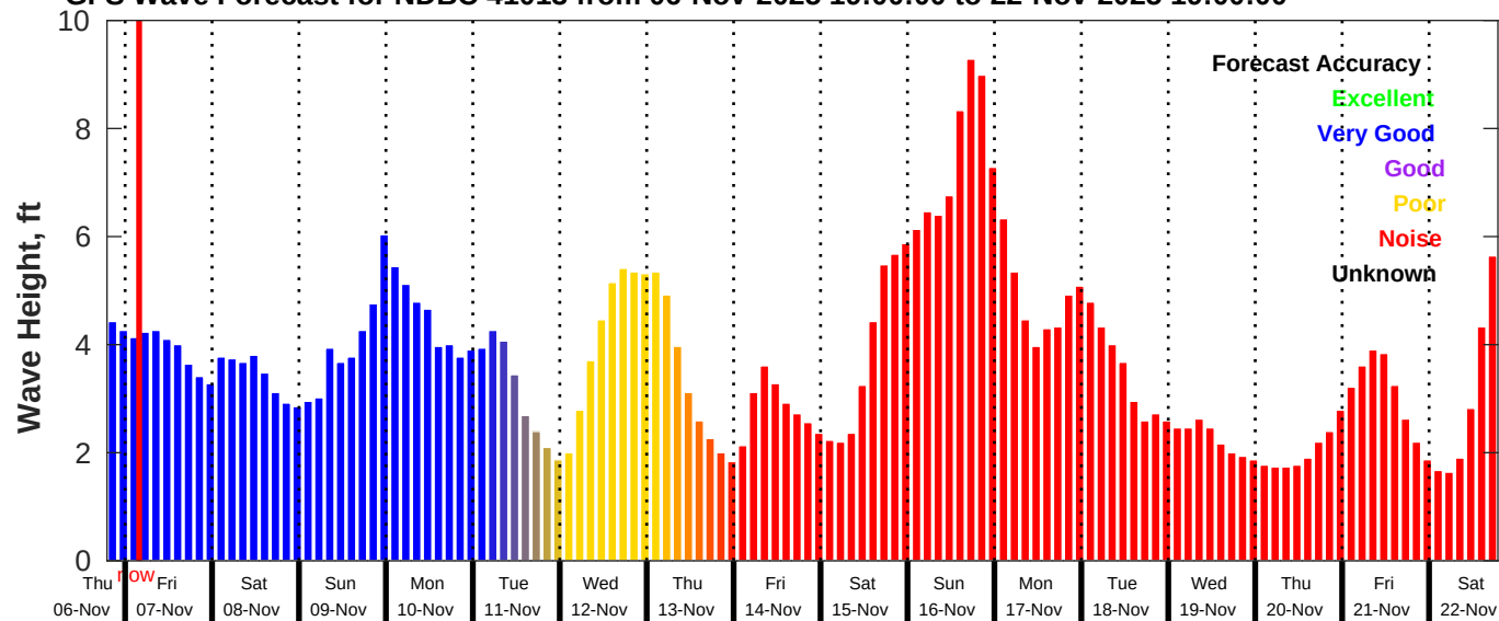
GFS Wave Forecast for NDBC 41013 from 06-Nov-2025 19:00:00 to 22-Nov-2025 19:00:00
