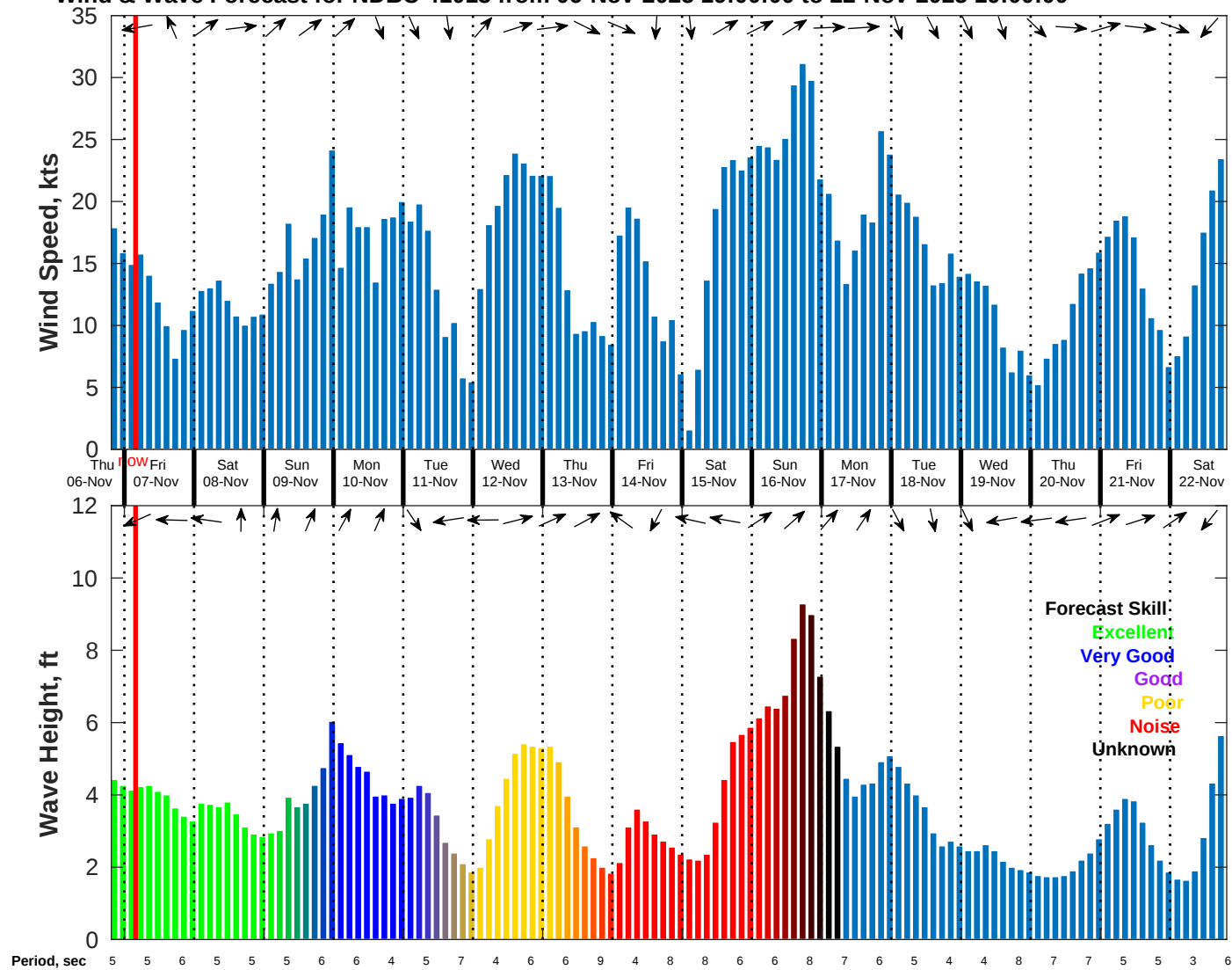
Wind & Wave Forecast for NDBC 41013 from 06-Nov-2025 19:00:00 to 22-Nov-2025 19:00:00
