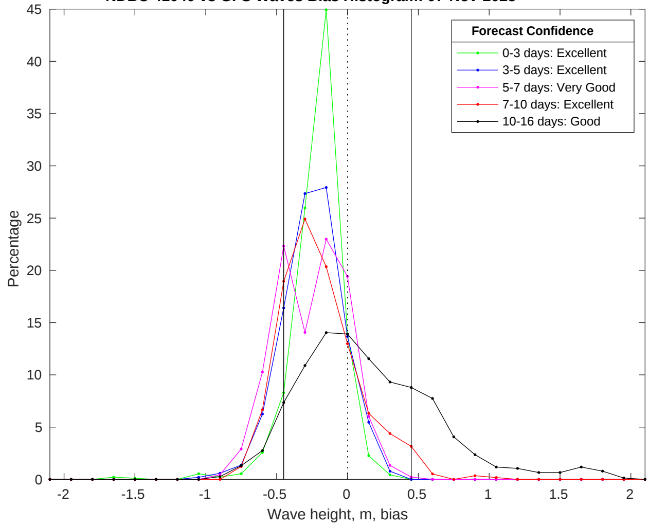
NDBC 41040 vs GFS Waves Bias Histogram: 07-Nov-2025
