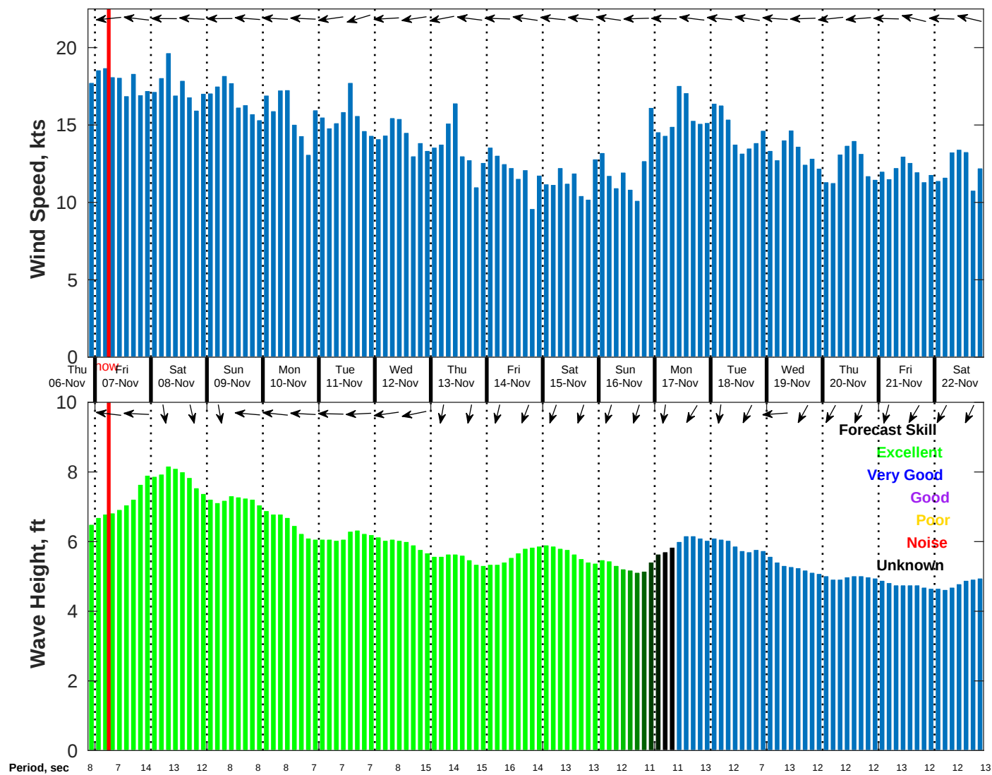
Wind & Wave Forecast for NDBC 41040 from 06-Nov-2025 21:00:00 to 22-Nov-2025 21:00:00
