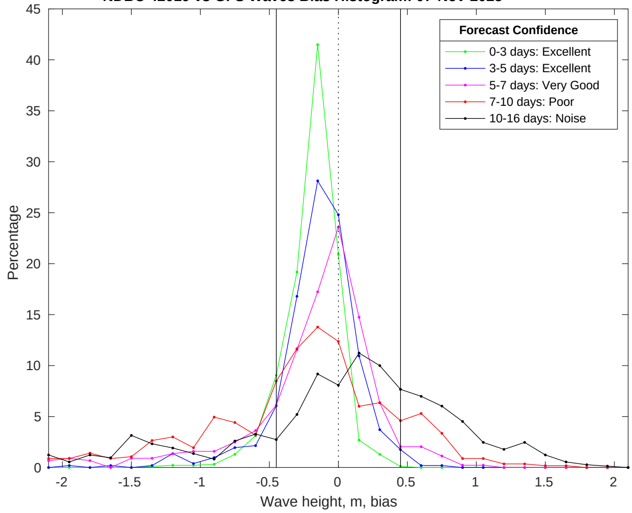
NDBC 42019 vs GFS Waves Bias Histogram: 07-Nov-2025
