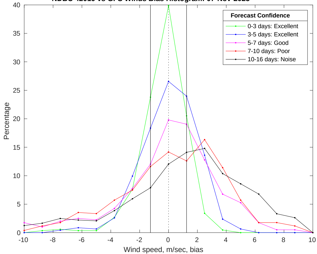
NDBC 42019 vs GFS Winds Bias Histogram: 07-Nov-2025
