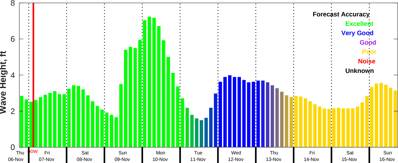
CMEMS Wave Forecast for NDBC 42019 from 06-Nov-2025 18:00:00 to 16-Nov-2025 18:00:00
