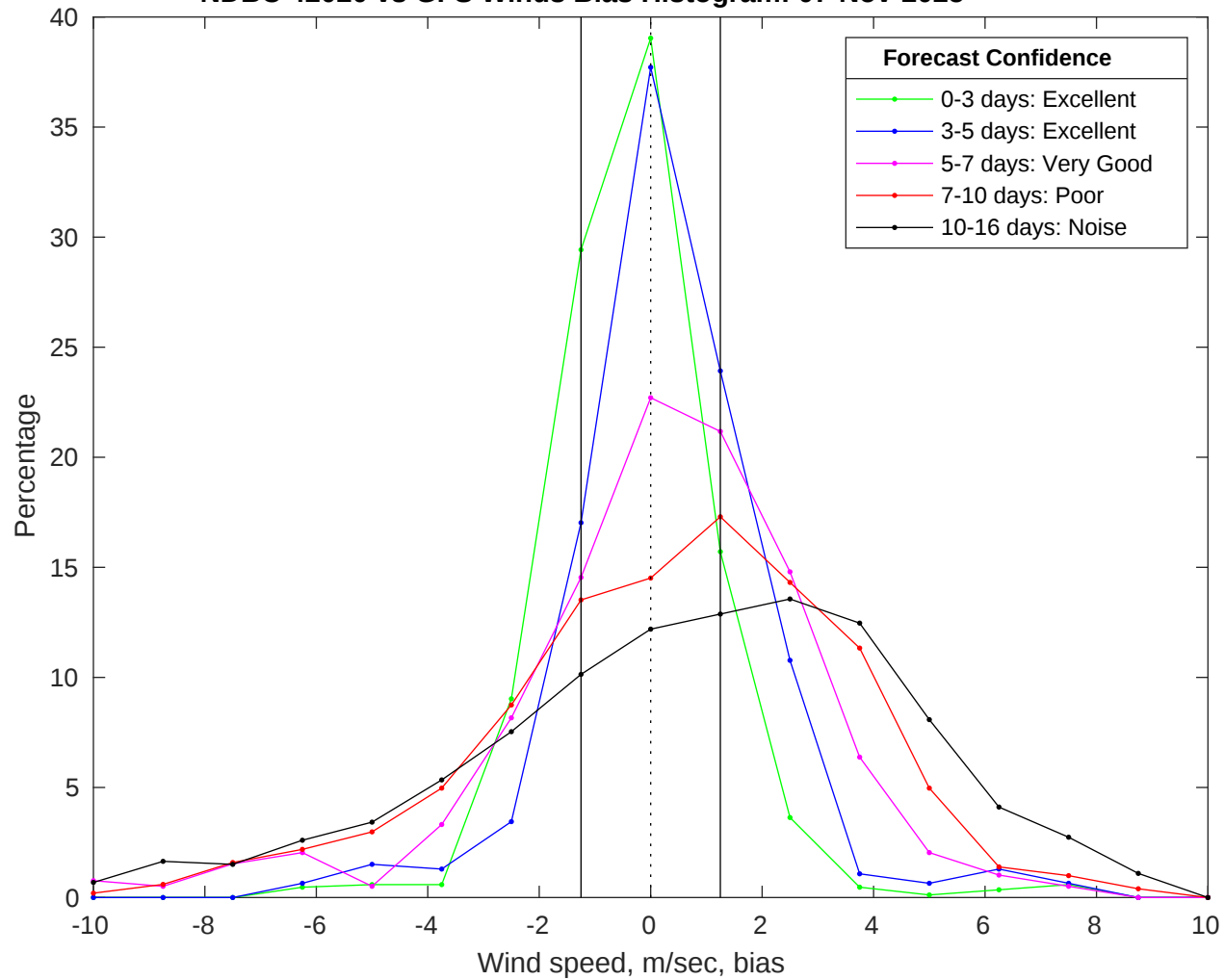
NDBC 42020 vs GFS Winds Bias Histogram: 07-Nov-2025
