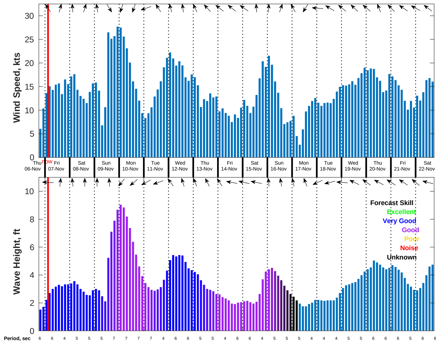
Wind & Wave Forecast for NDBC 42020 from 06-Nov-2025 18:00:00 to 22-Nov-2025 18:00:00
