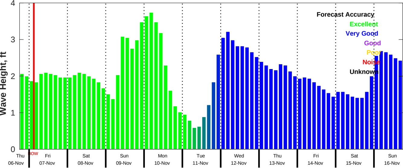
CMEMS Wave Forecast for NDBC 42035 from 06-Nov-2025 18:00:00 to 16-Nov-2025 18:00:00
