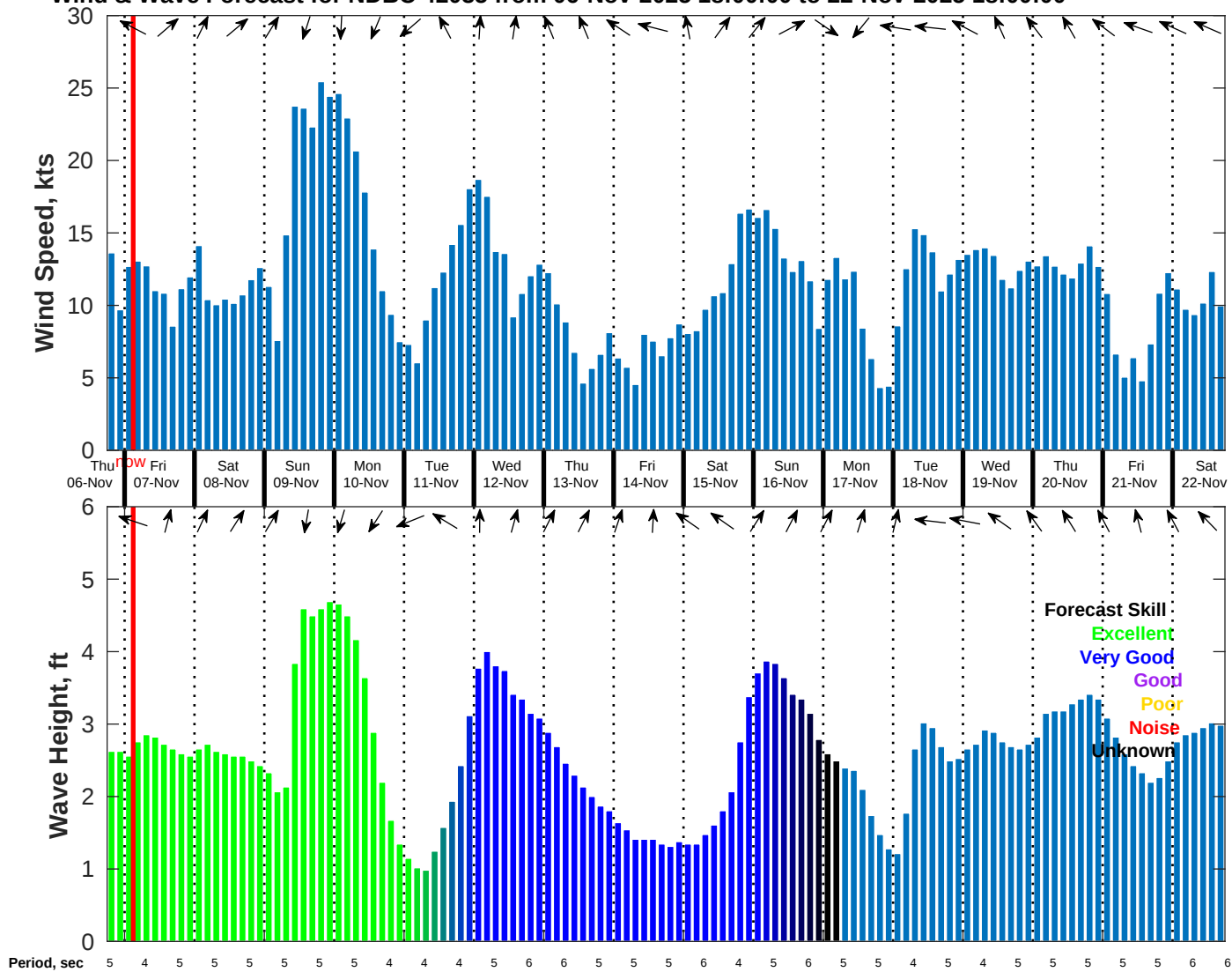
Wind & Wave Forecast for NDBC 42035 from 06-Nov-2025 18:00:00 to 22-Nov-2025 18:00:00
