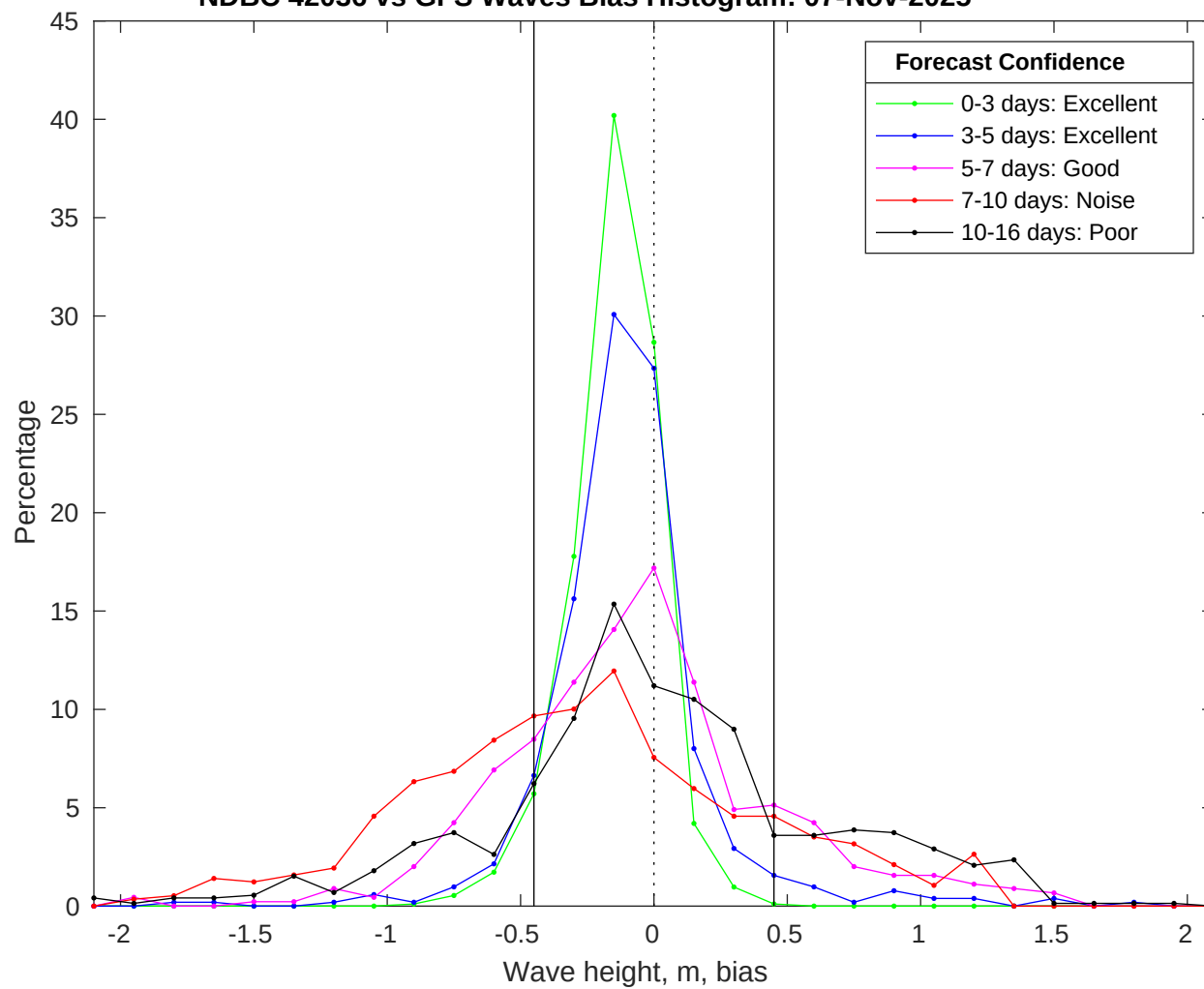
NDBC 42036 vs GFS Waves Bias Histogram: 07-Nov-2025
