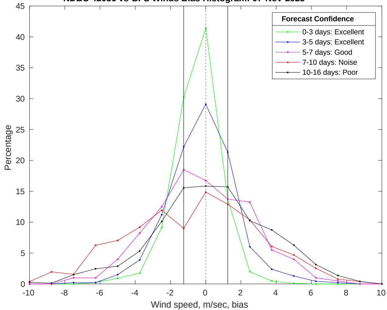
NDBC 42036 vs GFS Winds Bias Histogram: 07-Nov-2025
