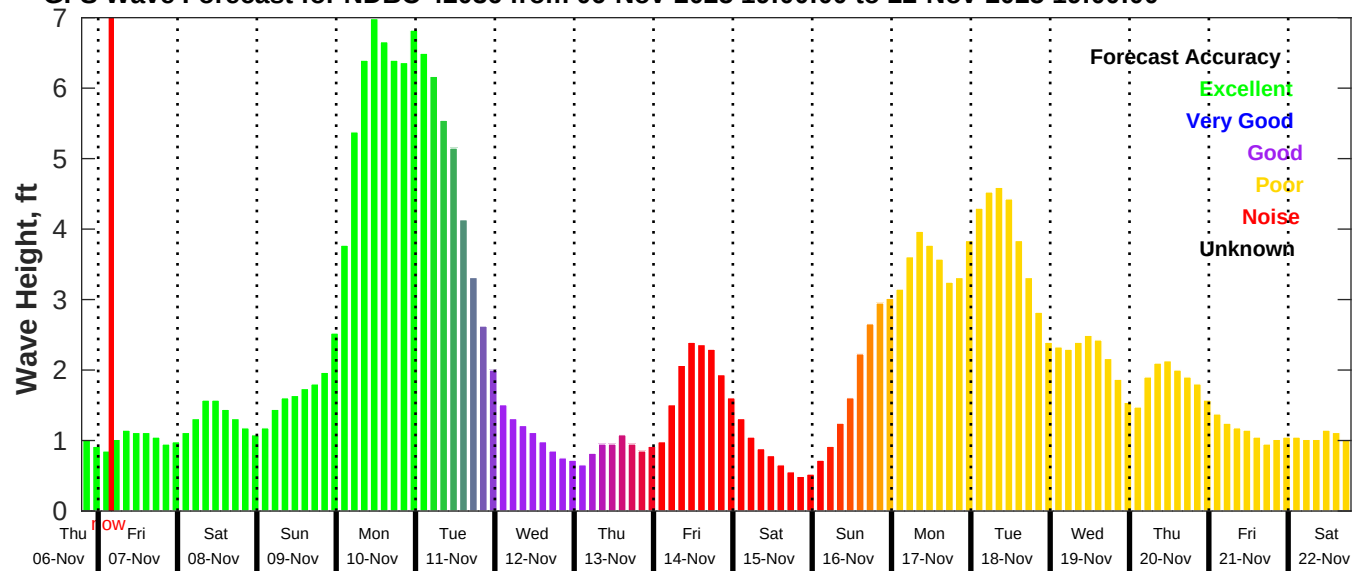
GFS Wave Forecast for NDBC 42036 from 06-Nov-2025 19:00:00 to 22-Nov-2025 19:00:00
