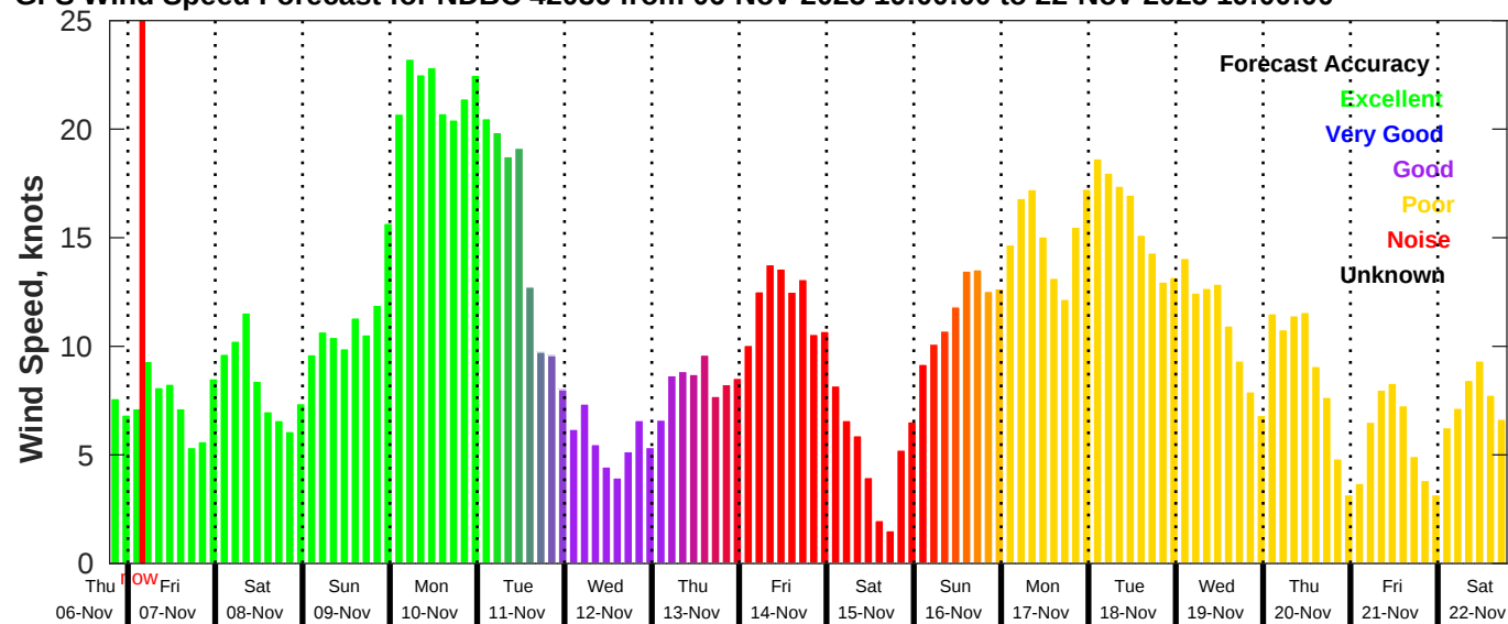
GFS Wind Speed Forecast for NDBC 42036 from 06-Nov-2025 19:00:00 to 22-Nov-2025 19:00:00
