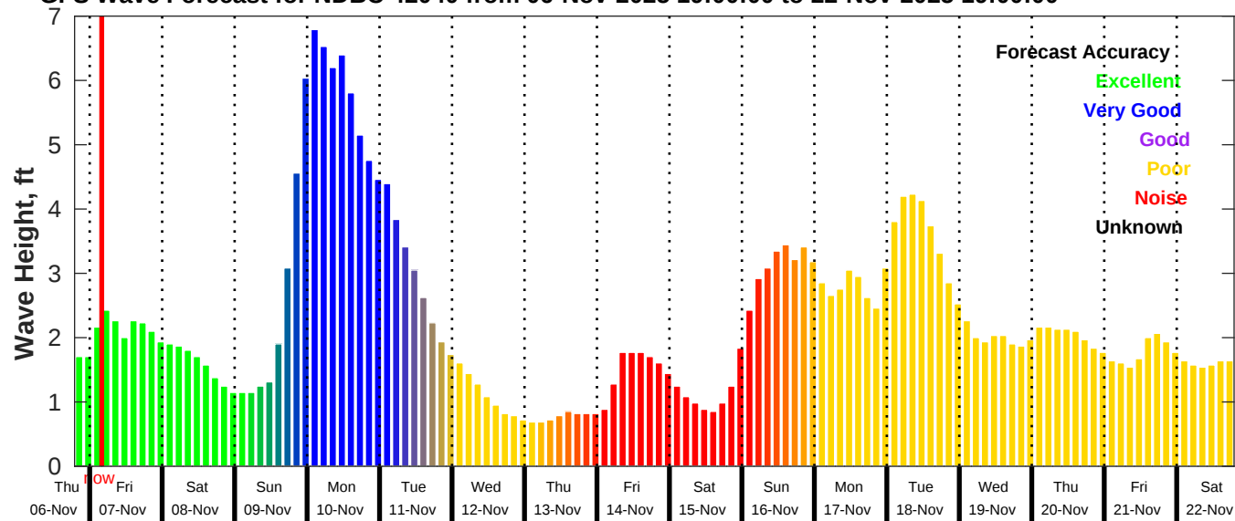
GFS Wave Forecast for NDBC 42040 from 06-Nov-2025 19:00:00 to 22-Nov-2025 19:00:00
