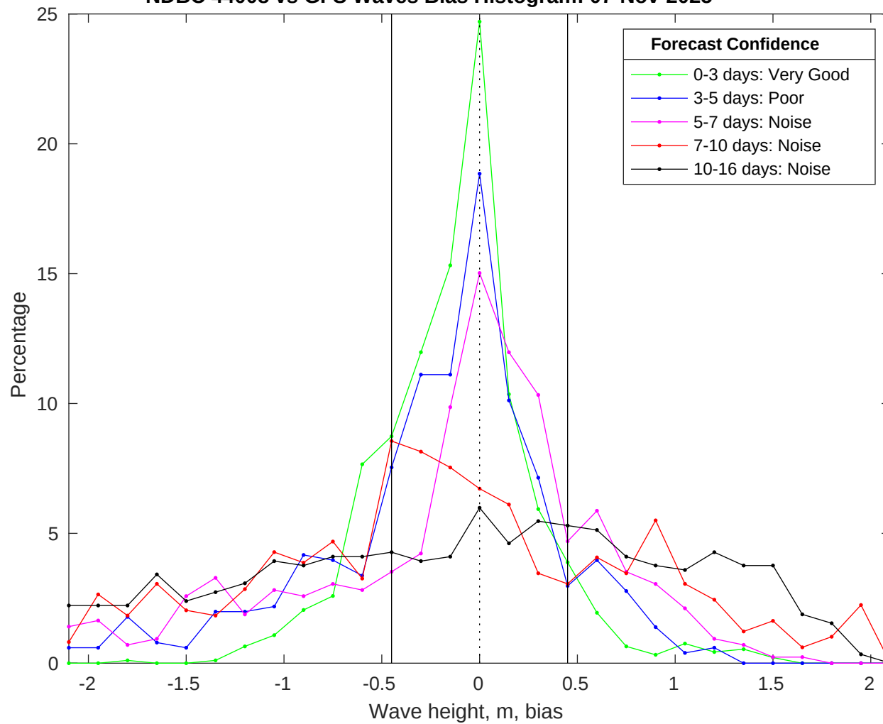
NDBC 44008 vs GFS Waves Bias Histogram: 07-Nov-2025
