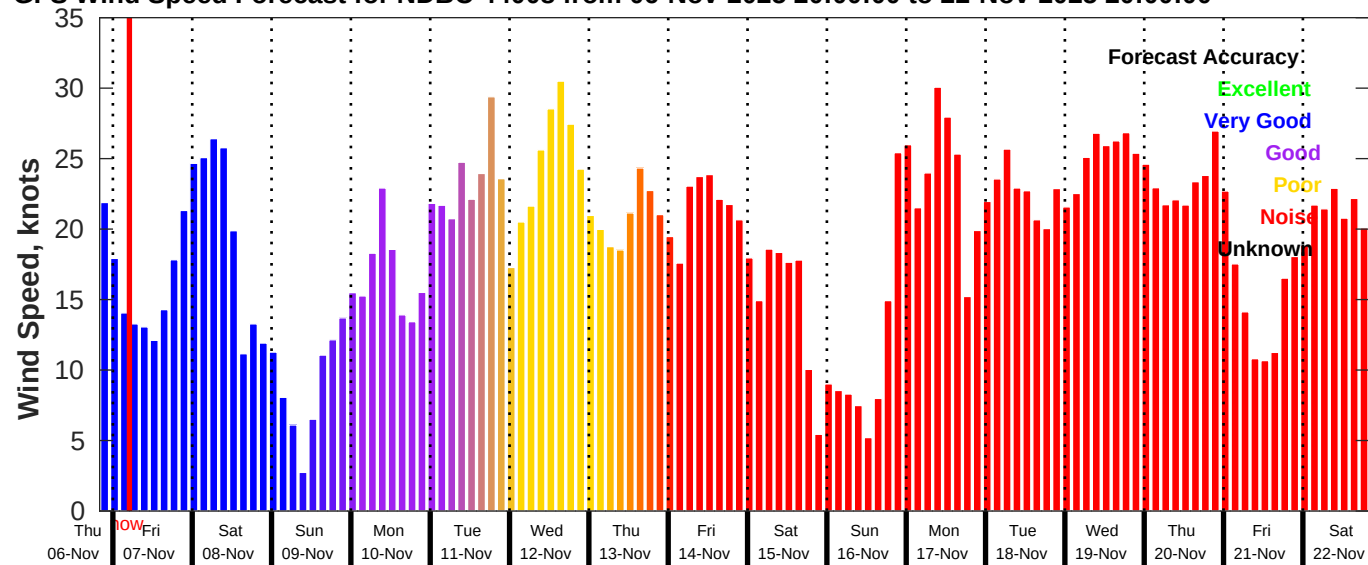
GFS Wind Speed Forecast for NDBC 44008 from 06-Nov-2025 20:00:00 to 22-Nov-2025 20:00:00
