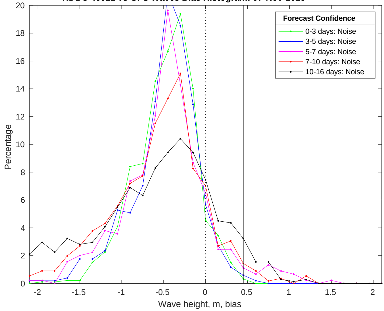
NDBC 46011 vs GFS Waves Bias Histogram: 07-Nov-2025
