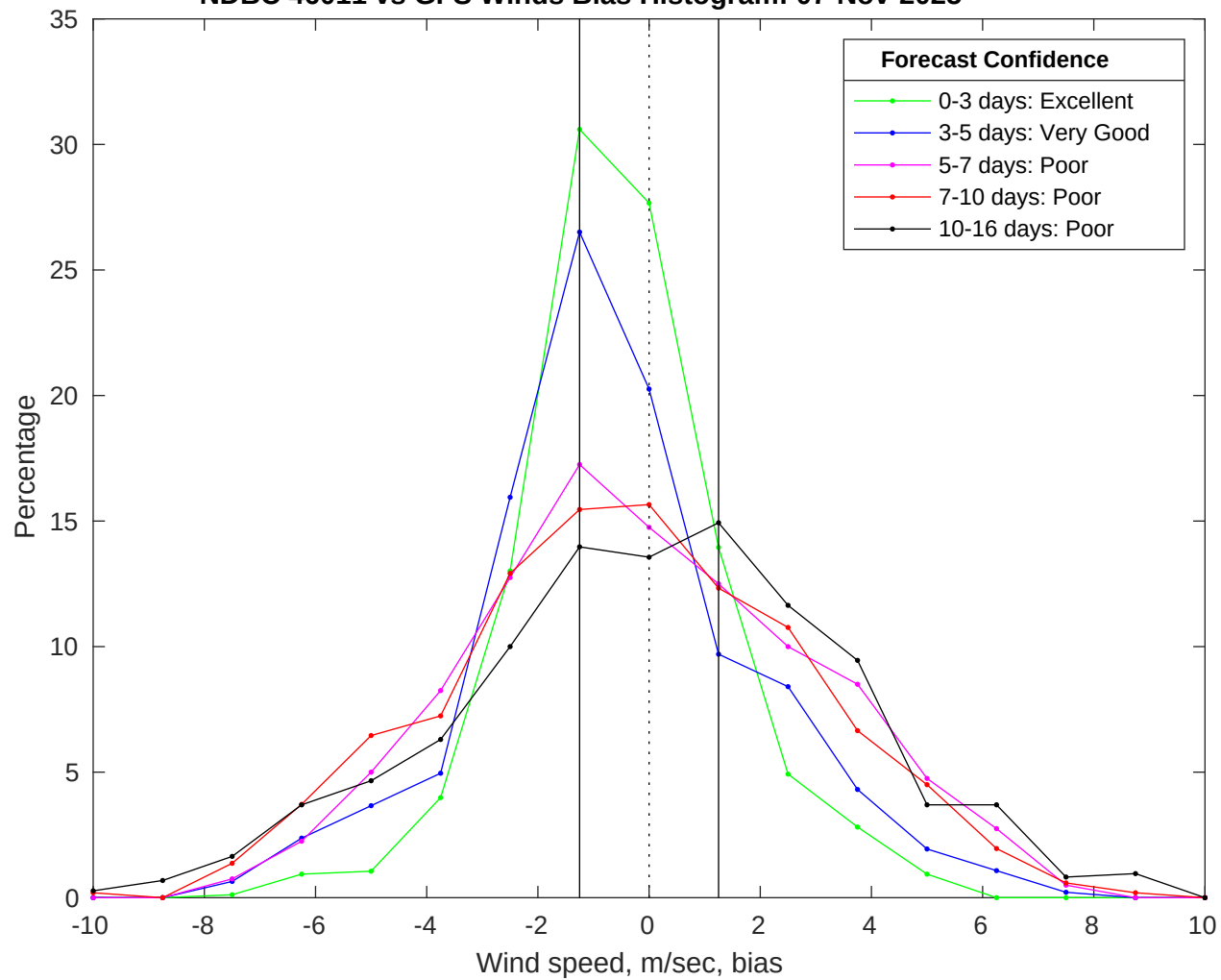
NDBC 46011 vs GFS Winds Bias Histogram: 07-Nov-2025
