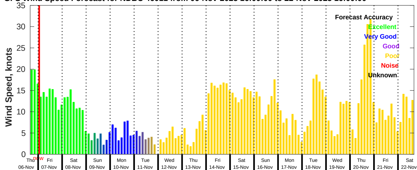
GFS Wind Speed Forecast for NDBC 46011 from 06-Nov-2025 16:00:00 to 22-Nov-2025 16:00:00
