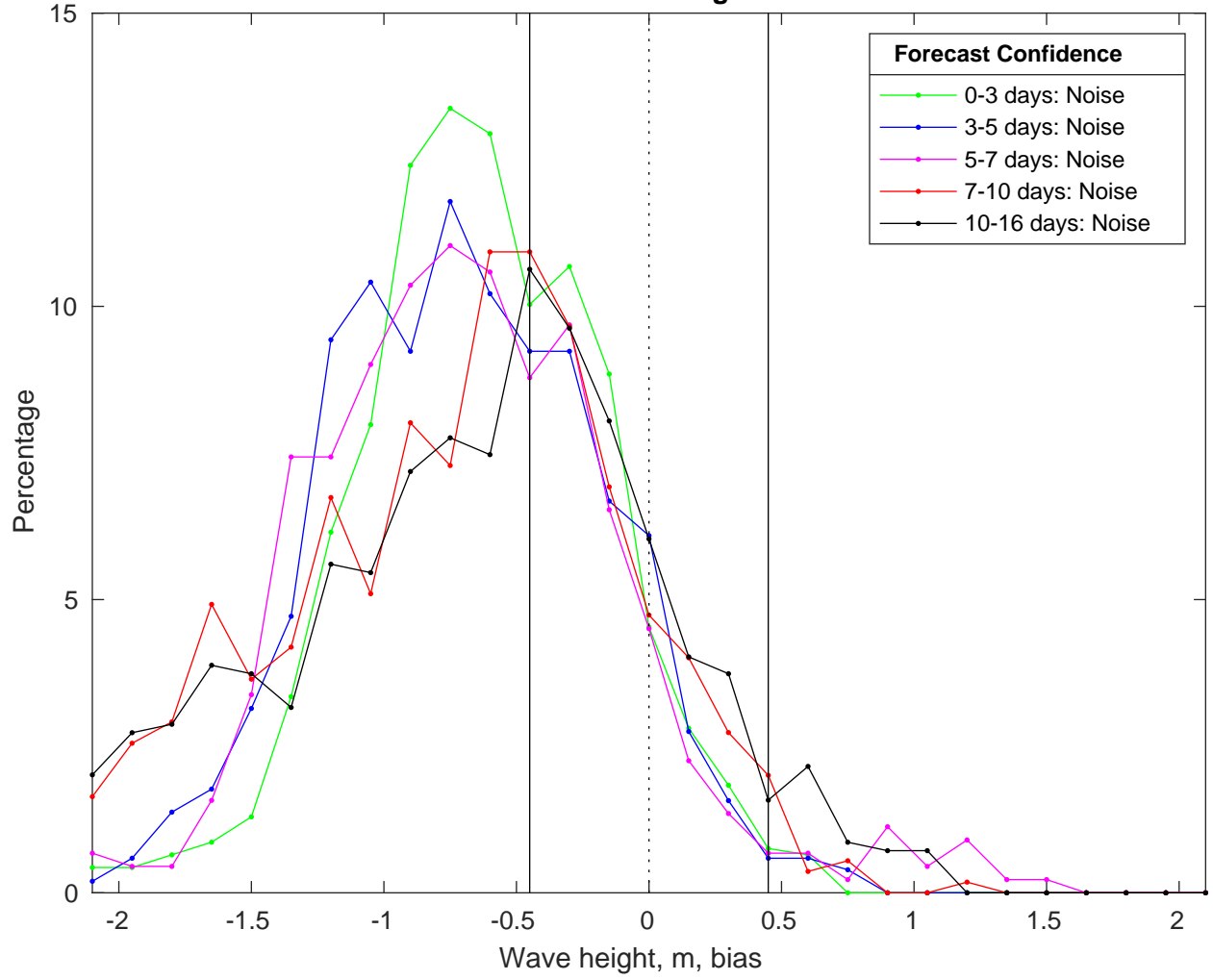
NDBC 46028 vs GFS Waves Bias Histogram: 07-Nov-2025
