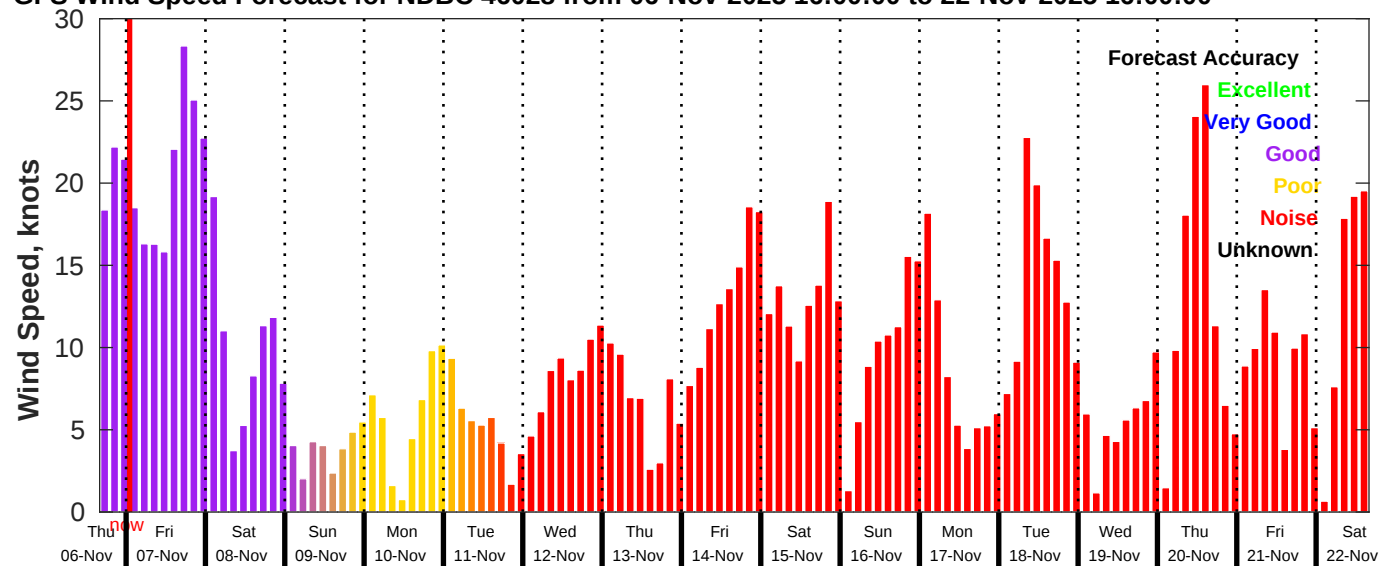
GFS Wind Speed Forecast for NDBC 46028 from 06-Nov-2025 16:00:00 to 22-Nov-2025 16:00:00
