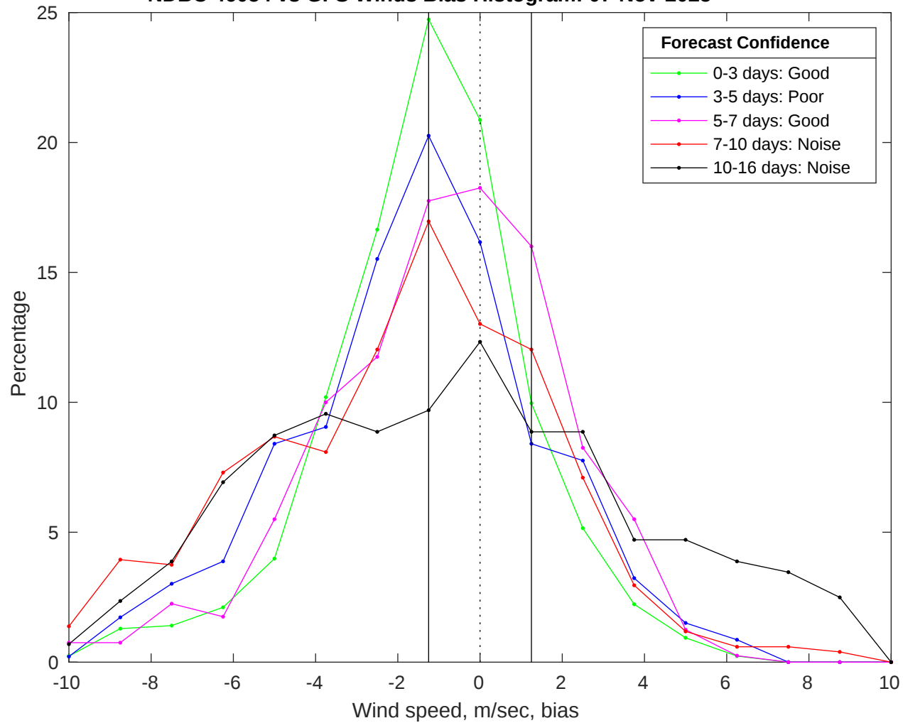
NDBC 46054 vs GFS Winds Bias Histogram: 07-Nov-2025
