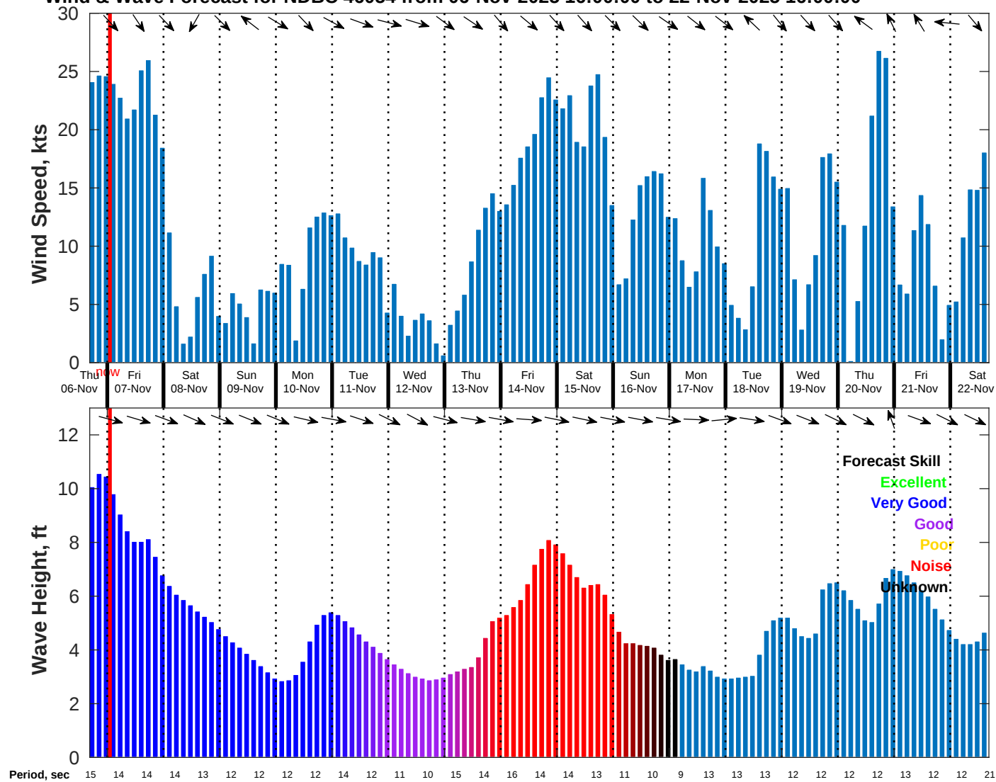
Wind & Wave Forecast for NDBC 46054 from 06-Nov-2025 16:00:00 to 22-Nov-2025 16:00:00
